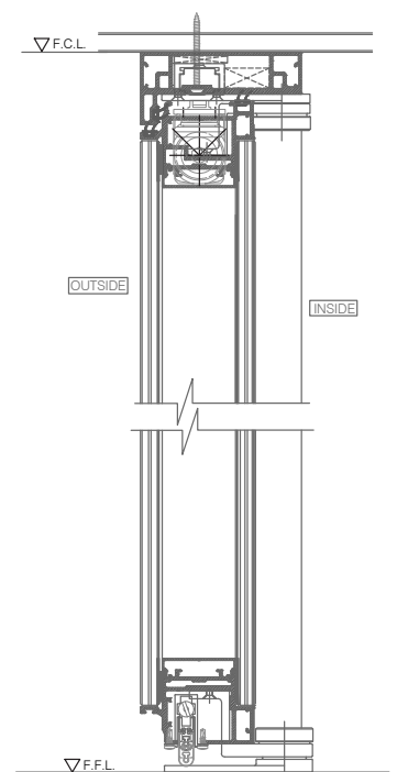
VERTICAL SECTION
