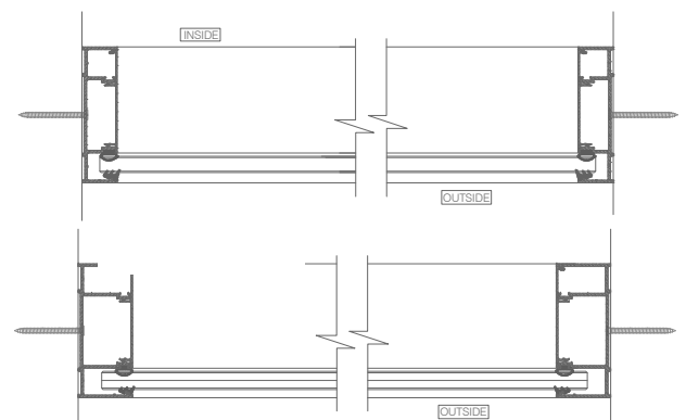
HORIZONTAL SECTION
