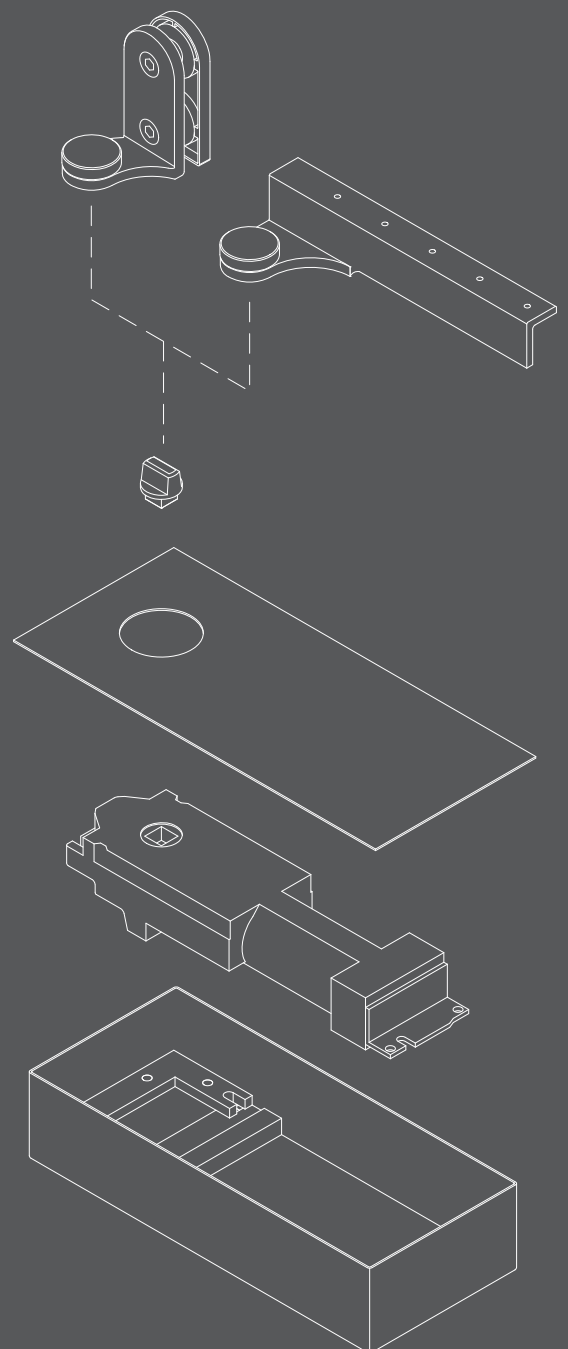
Concealed floor spring option for JEB hinges
